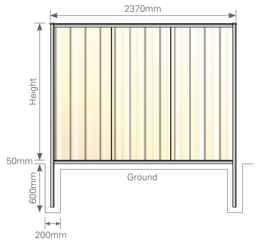
TL-5 rail
