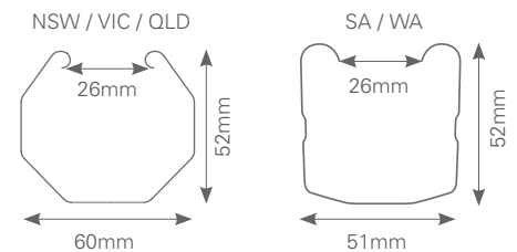
TL-5 rail
